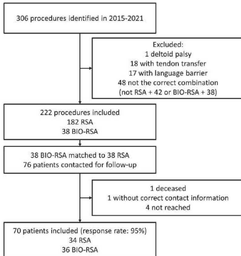
Figure 1: Inclusion flowchart
